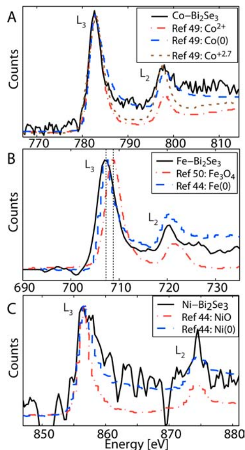
Figure 7. EELS spectra of Co, Fe, Ni intercalated Bi 2 Se 3 nanoribbons plotted with reference spectra, 44,49,50 confirm that intercalated metals are zerovalent by the ratio of the L 3 to L 2 edges and spectral shape and position.
